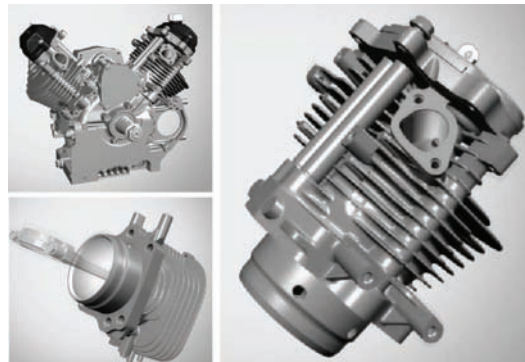
Integrated cylinder and head structure
